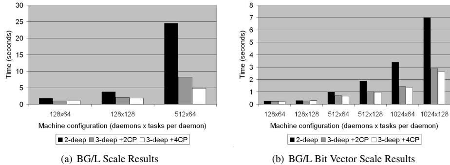
Figure 4. BG/L scale STATBench performance results with (a) string-based task lists and (b) bit vector task lists.
