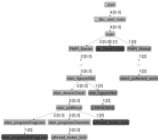
Figure 1. An example 3D-Trace/Space/Time call graph prefix tree from STAT.
